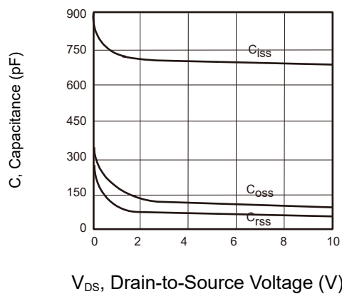
Figure 3: Capacitance
