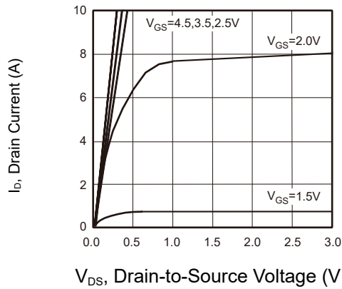
Fig 1: On-Region Characteristics
