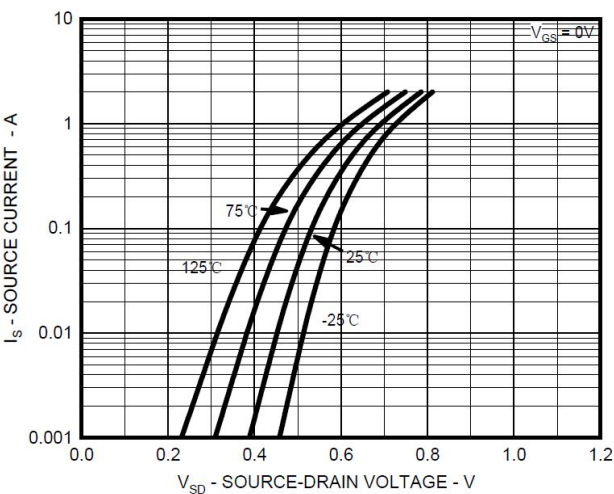
Fig.4 Diode Forward Voltage vs. Current
