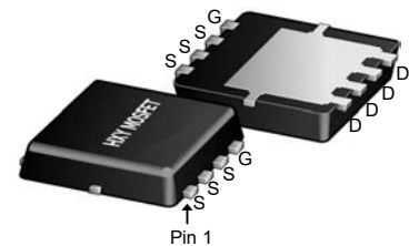
DFN5X6-8L (DFN-8(4.9x5.8))
