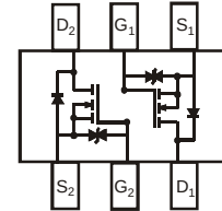
Internal Schematic
