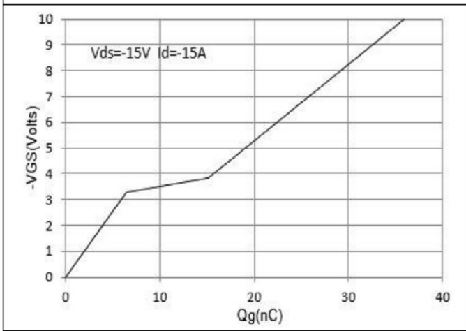
Figure 7. Gate-Charge Characteristics
