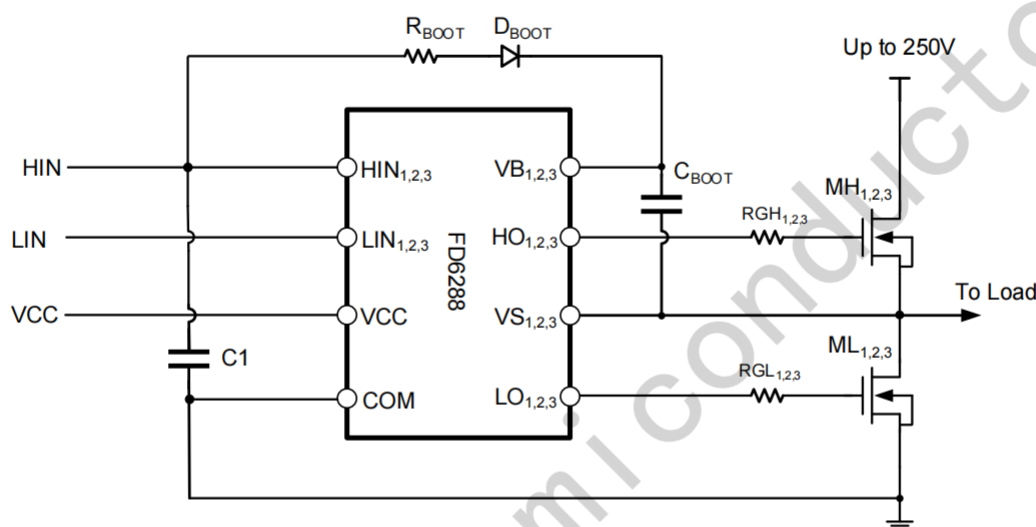
Figure8-1 Typical application circuit of FD6288
