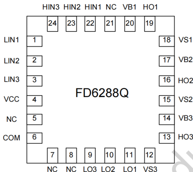
Figure4-2 24-Pin QFN Top view
