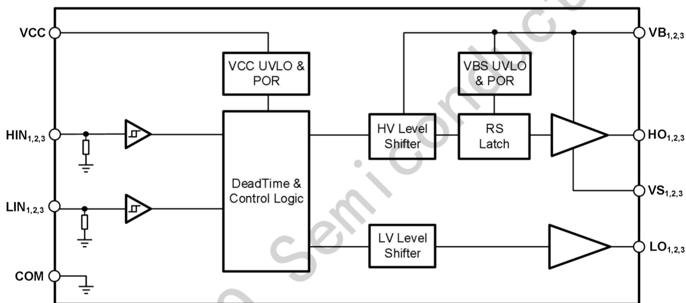
Figure7-1 Function Block Diagram of FD6288
