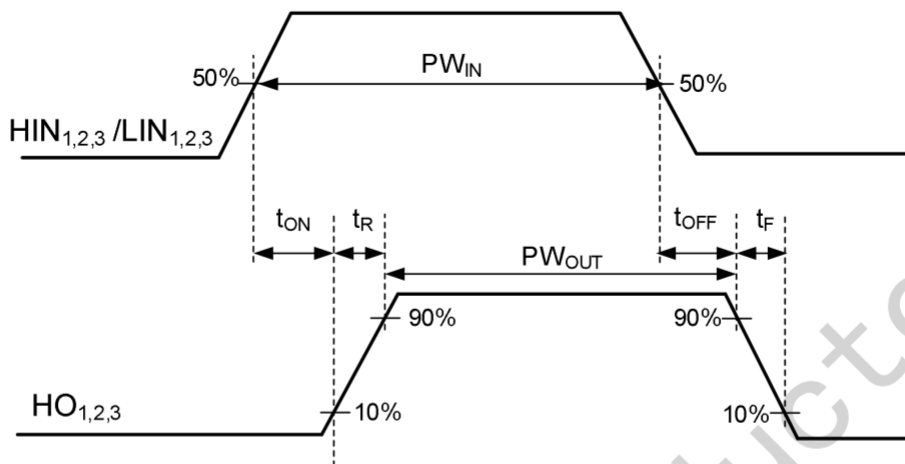
Figure 6-1 FD6288 Input and output timing waveform
