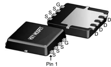
DFN5X6-8L (PQFN-8(4.9x5.8))
