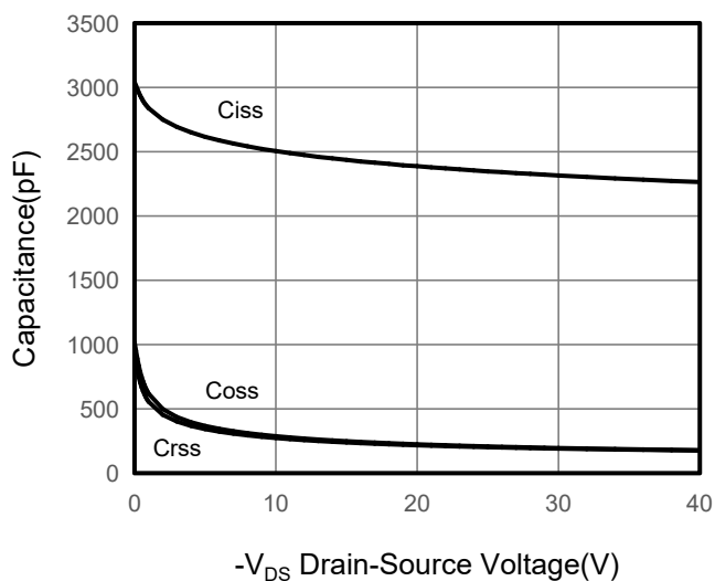
Figure 5. Capacitance
