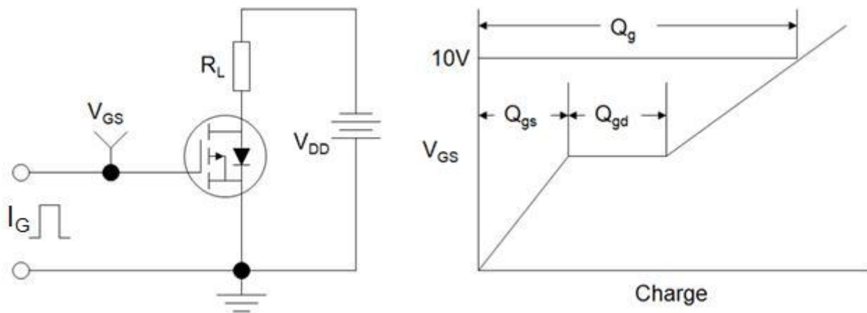
Gate Charge Test Circuit
