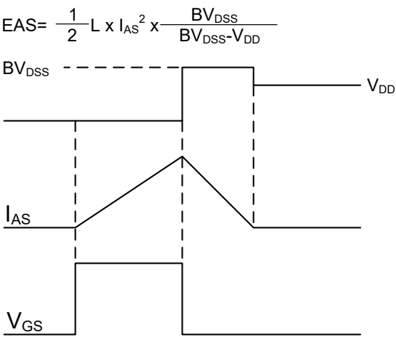
Fig.8 EAS Waveform
