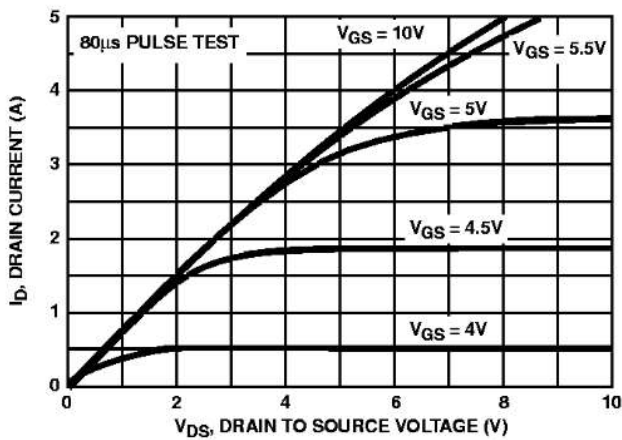
FIGURE 6. SATURATION CHARACTERISTICS
