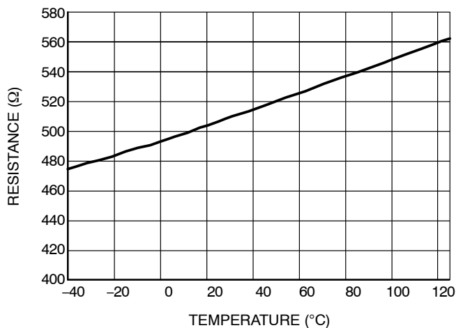
Figure 22. R_{t\_discharge}
