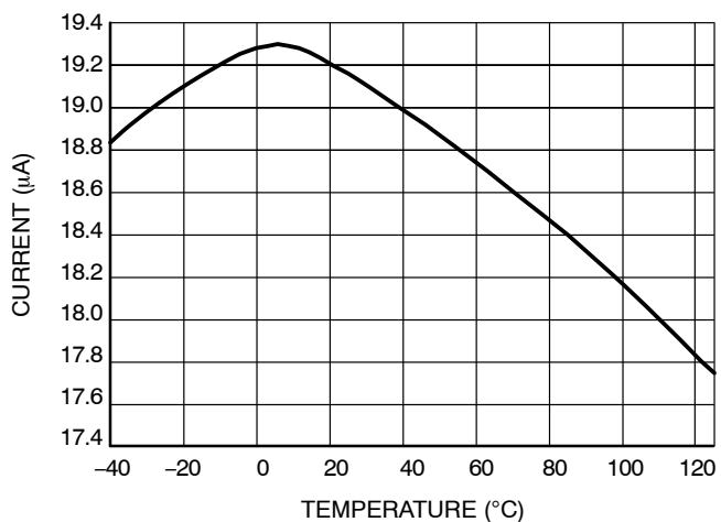
Figure 24. I_{BO}
