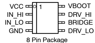
8 Pin Package
