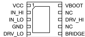
10 Pin DFN Package
