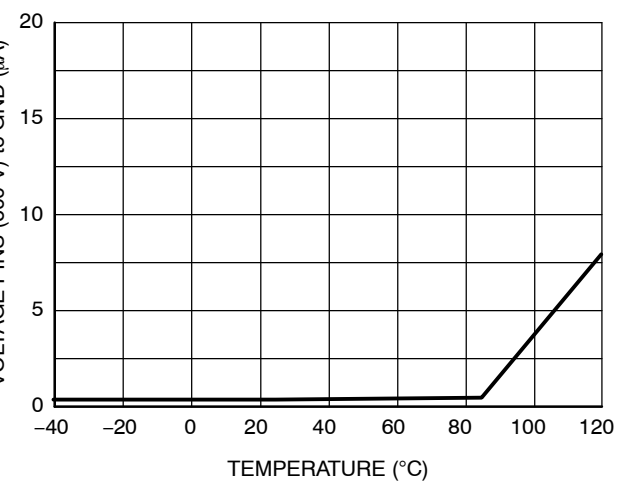
Figure 37. Leakage Current on High Voltage Pins (600 V) to Ground vs. Temperature ( V_{BRIDGE} = V_{BOOT} = V_{DRV\_HI} = 600\text{ V} )
