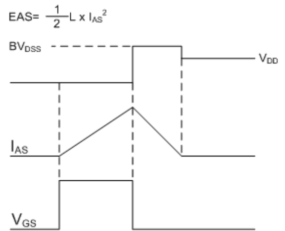
Fig.12 Unclamped Inductive Switching Test Circuit & Waveforms
