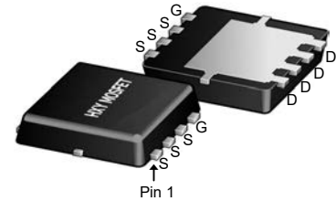
DFN5X6-8L (WPAK-8)
