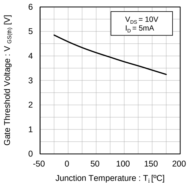
Fig.13 Gate Threshold Voltage vs. Junction Temperature
