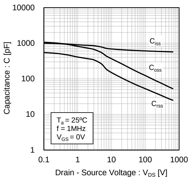
Fig.19 Typical Capacitance vs. Drain - Source Voltage
