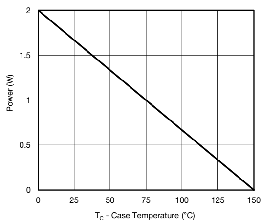
Power Junction-to-Foot
