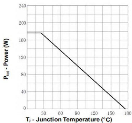
Fig 9. Power Dissipation
