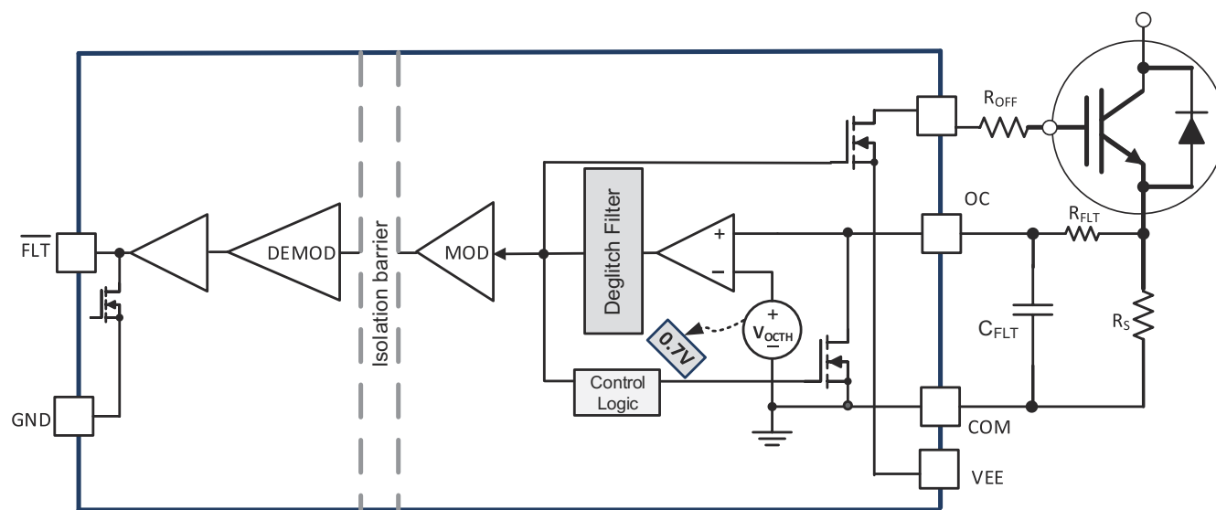
图 9-9. Overcurrent and Short Circuit Protection Based on Shunt Resistor
