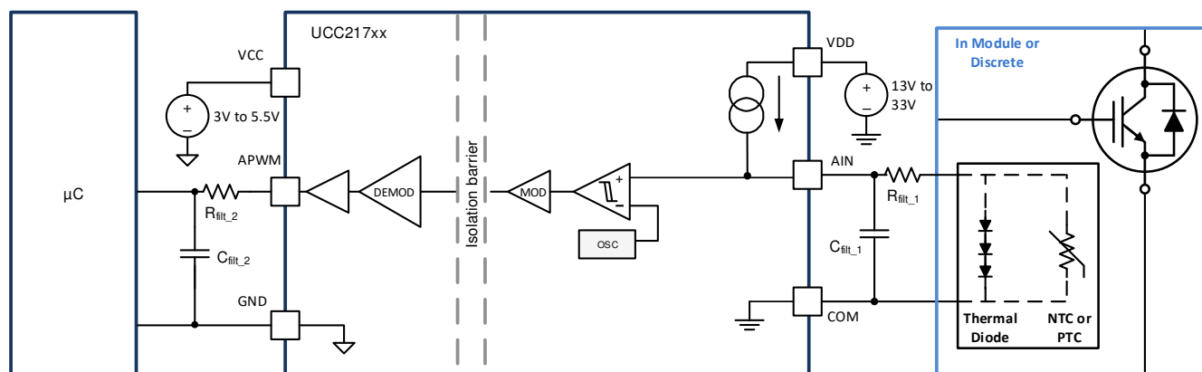
图 9-11. APWM Channel with Filtered Output
